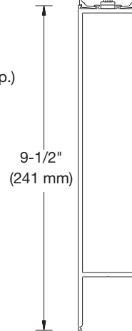
Special Bottom Rail to Comply With A.D.A.
